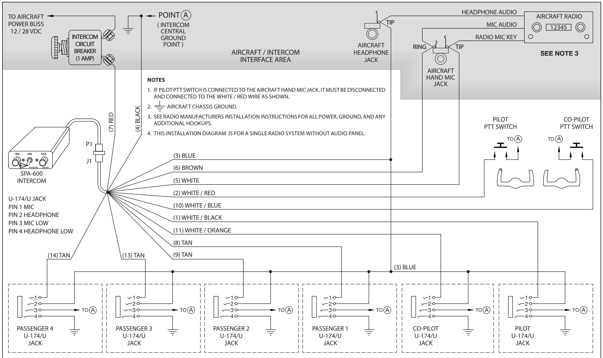
SPA-600 With U-174/U Jacks Installation Wiring Diagram
