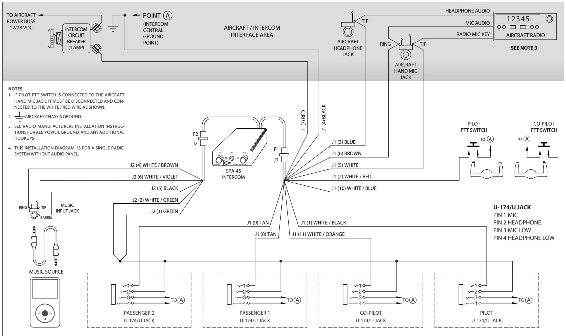
SPA-4S With U-174/U Jacks Installation Wiring Diagram
