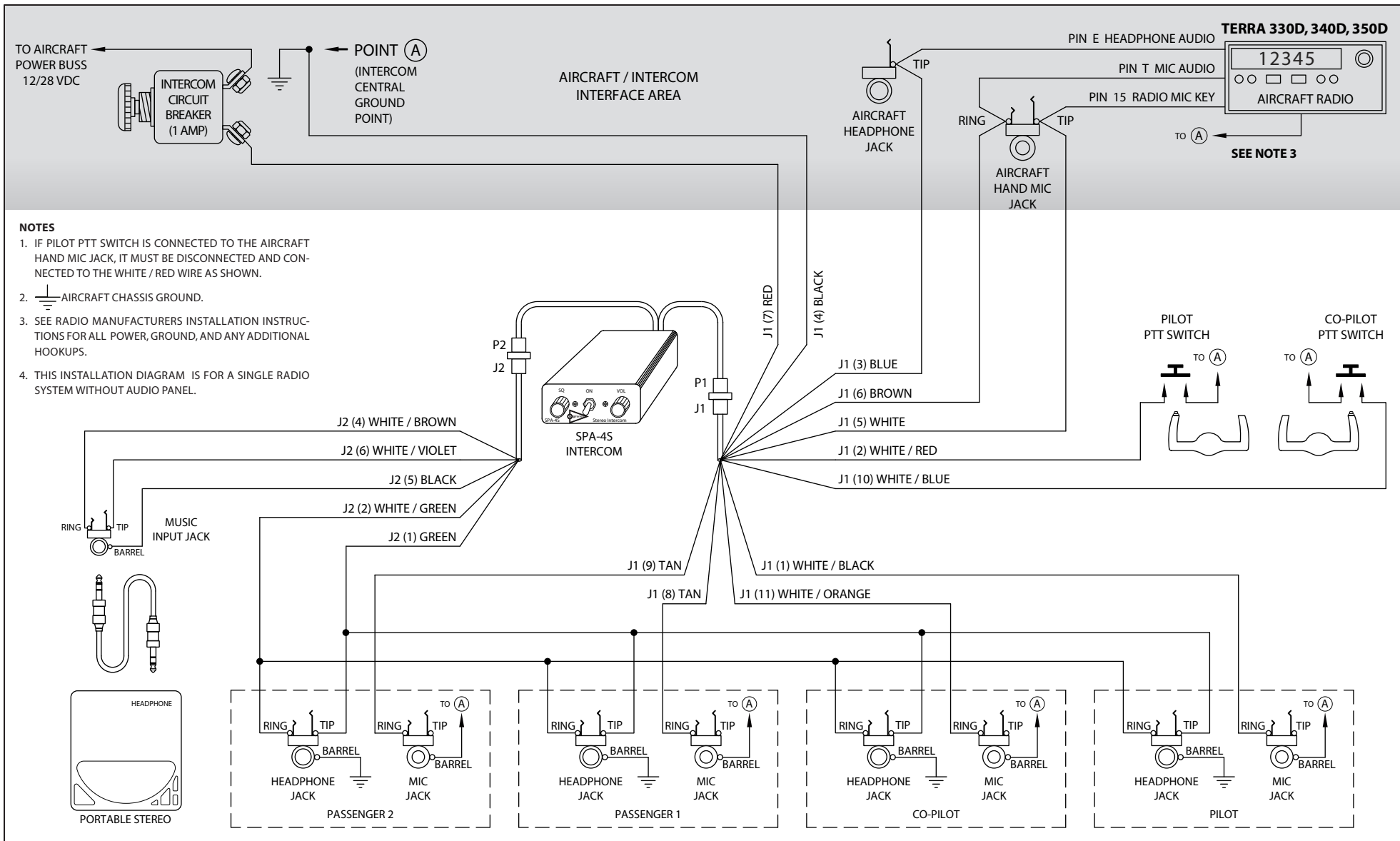
SPA-4S – TERRA TMA 330D, 340D, 350D Radio Installation Wiring Diagram
