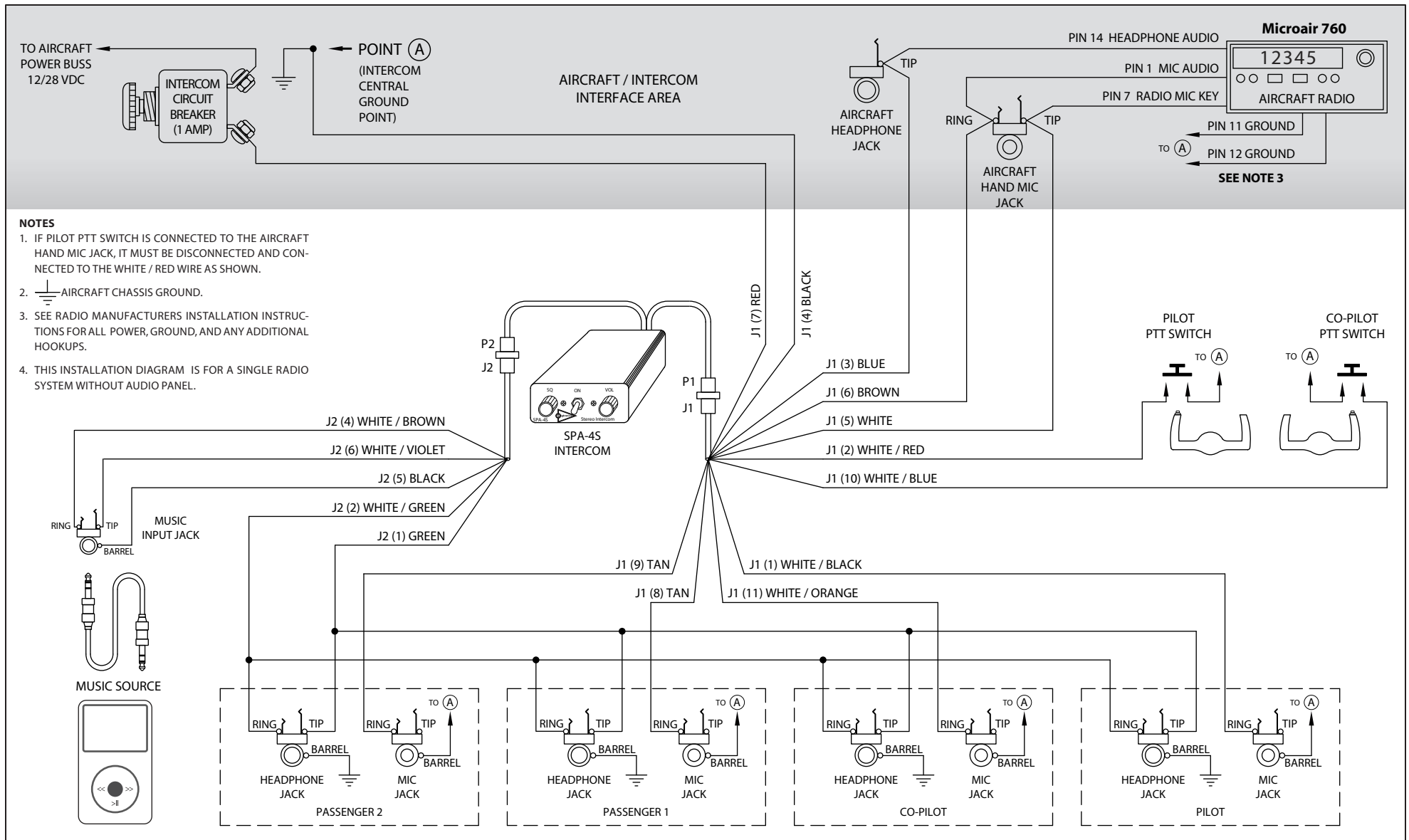
SPA-4S – Microair 760 Radio Installation Wiring Diagram
