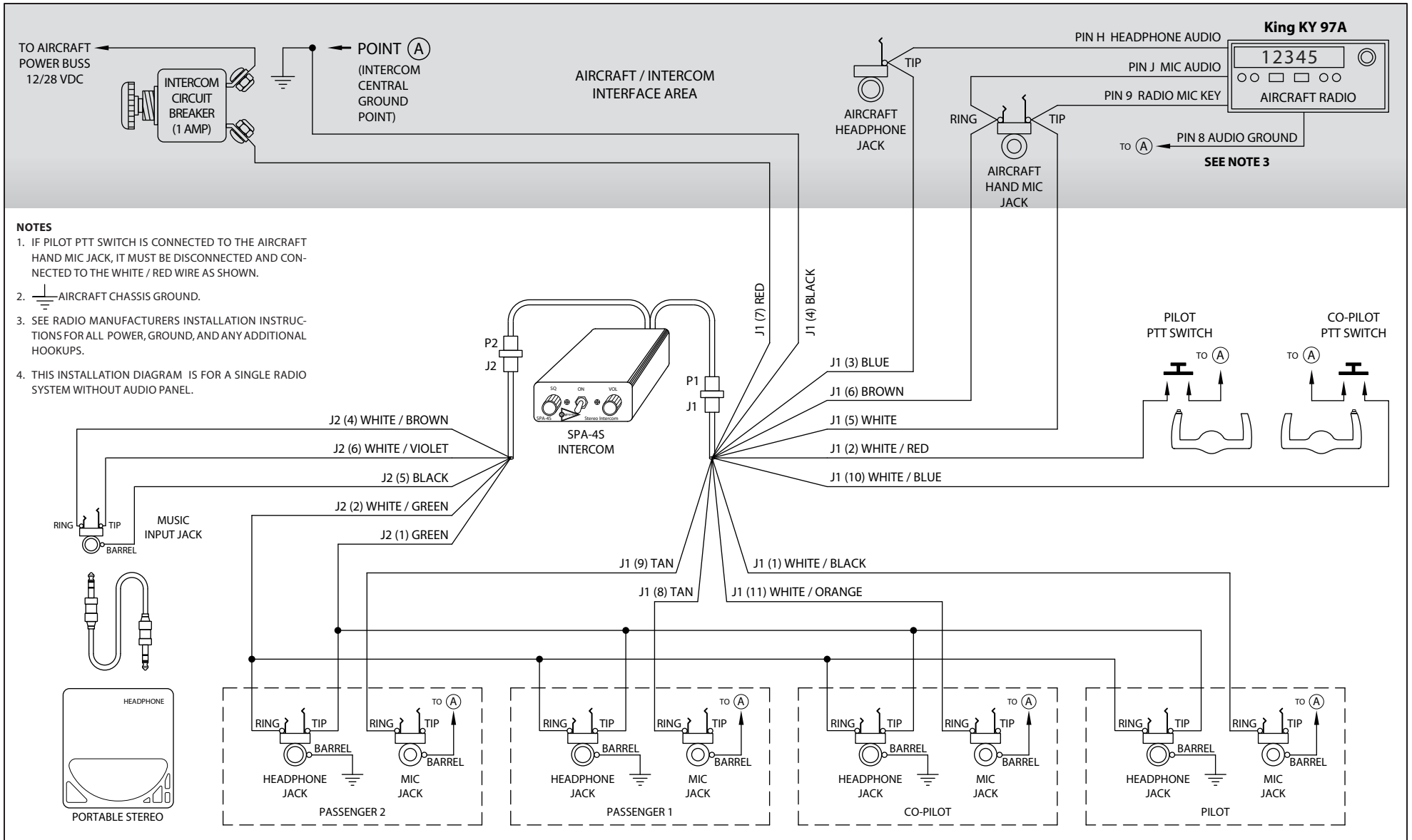
SPA-4S – King KY 97A Radio Installation Wiring Diagram
