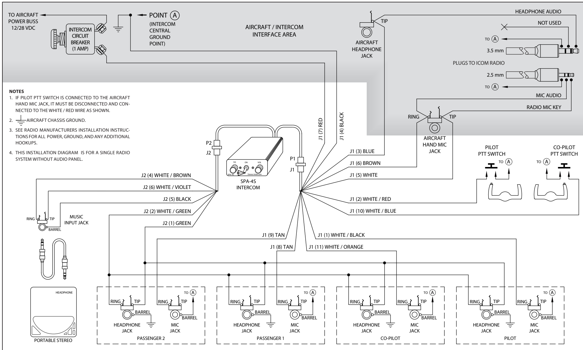
SPA-4S – ICOM A3, A6, A22, A24 Radio Installation Wiring Diagram
