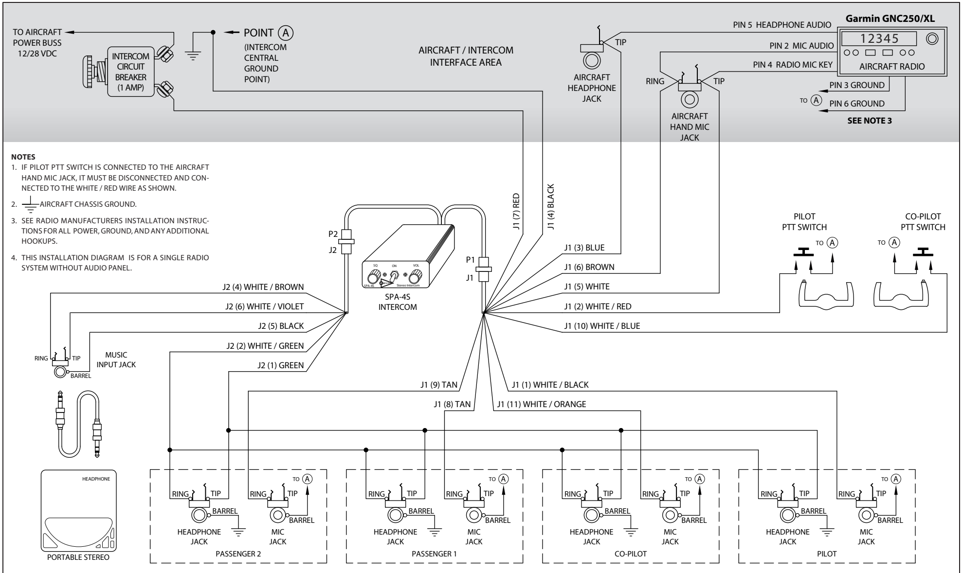
SPA-4S – Garmin GNC250/XL Radio Installation Wiring Diagram
