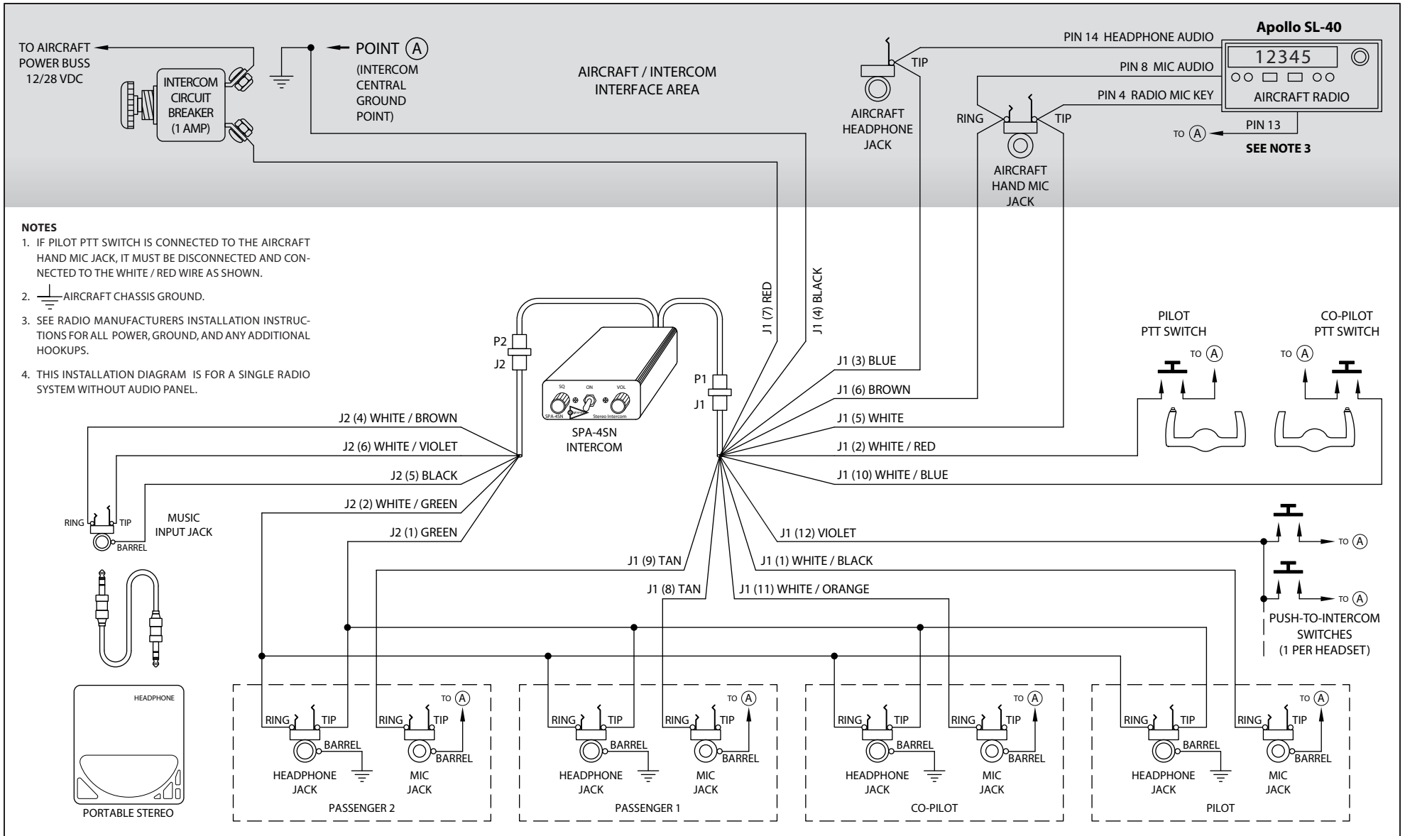
SPA-4SN – Apollo SL-40 Radio Installation Wiring Diagram
