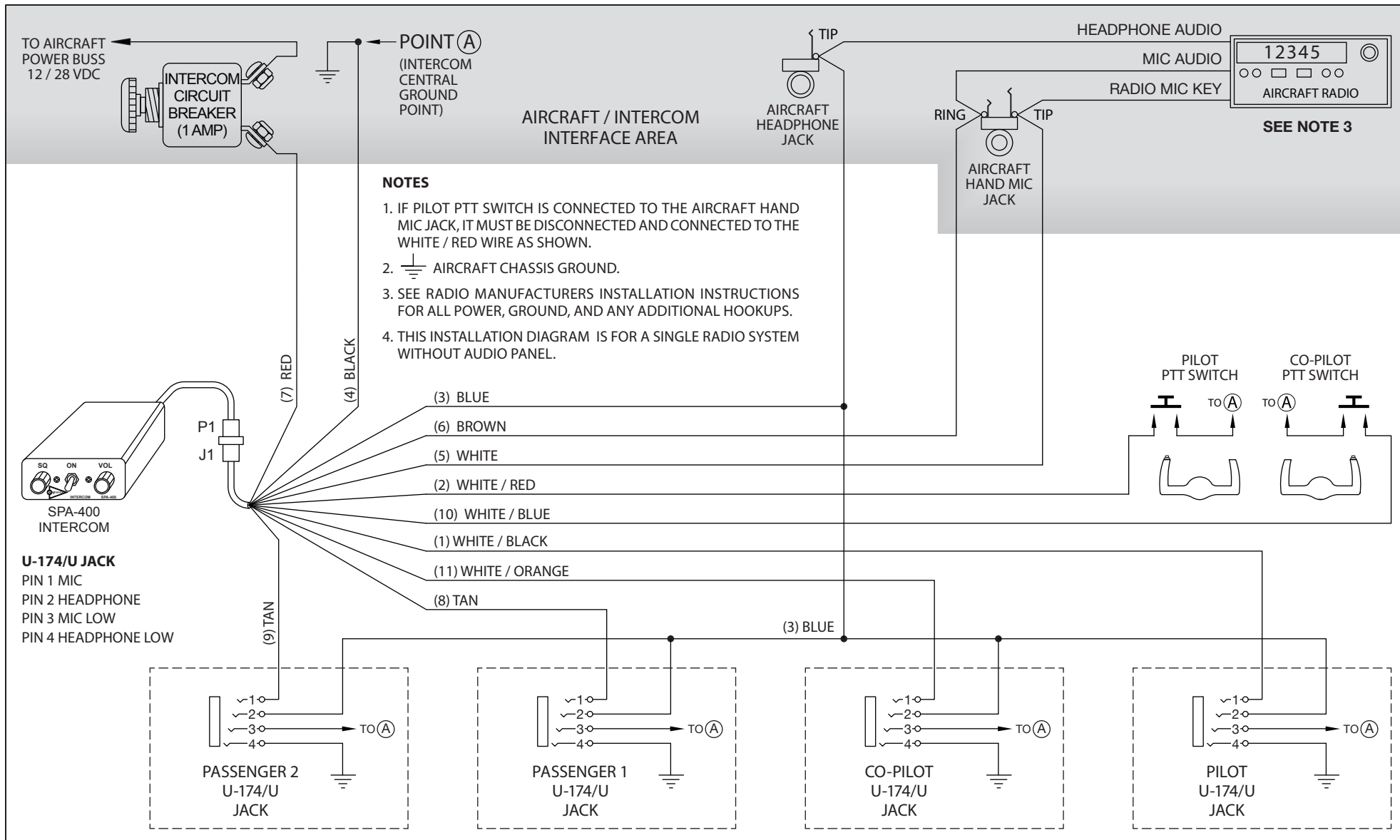
SPA-400 With U-174/U Jacks Installation Wiring Diagram
