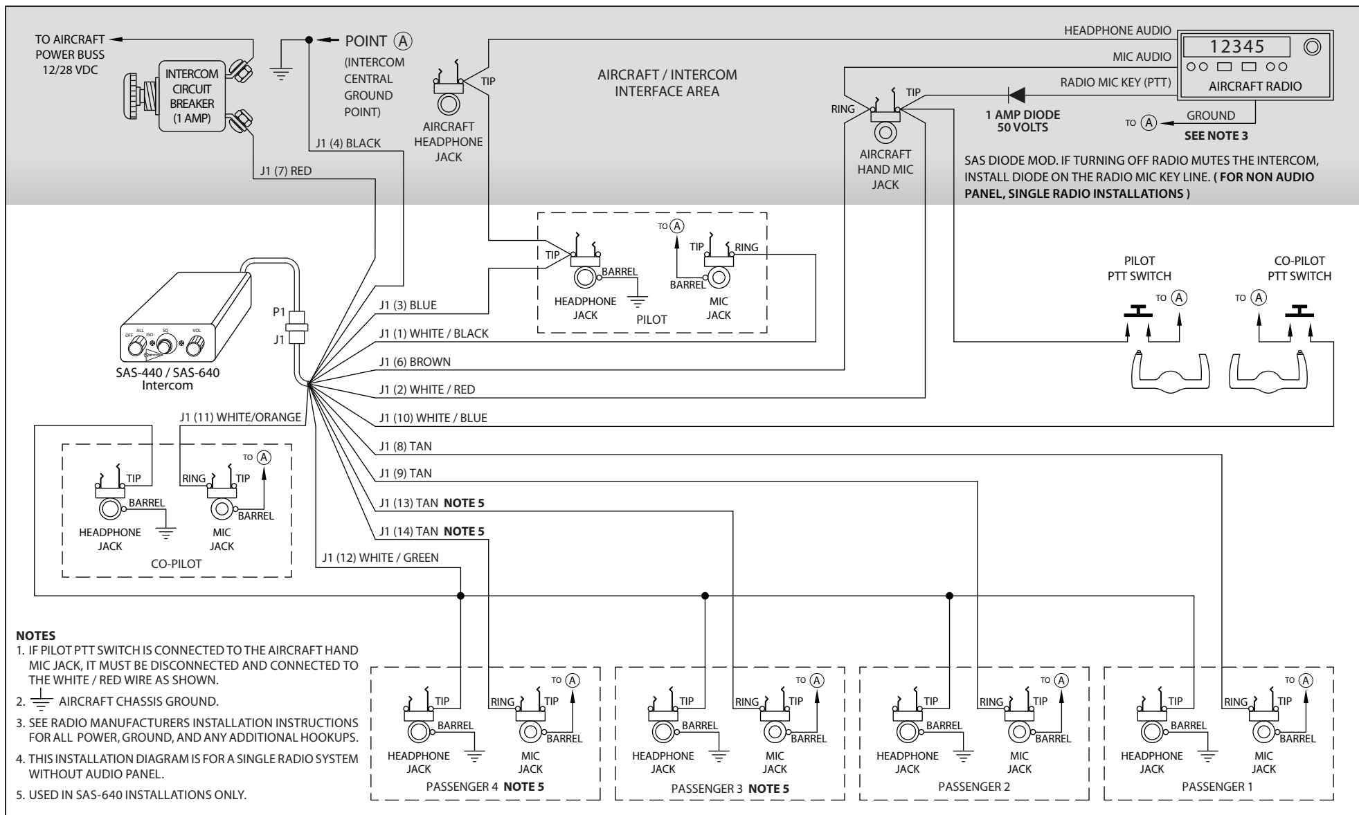
SAS-440 / SAS-640 – No Audio Panel (Single Radio) Installation Wiring Diagram
