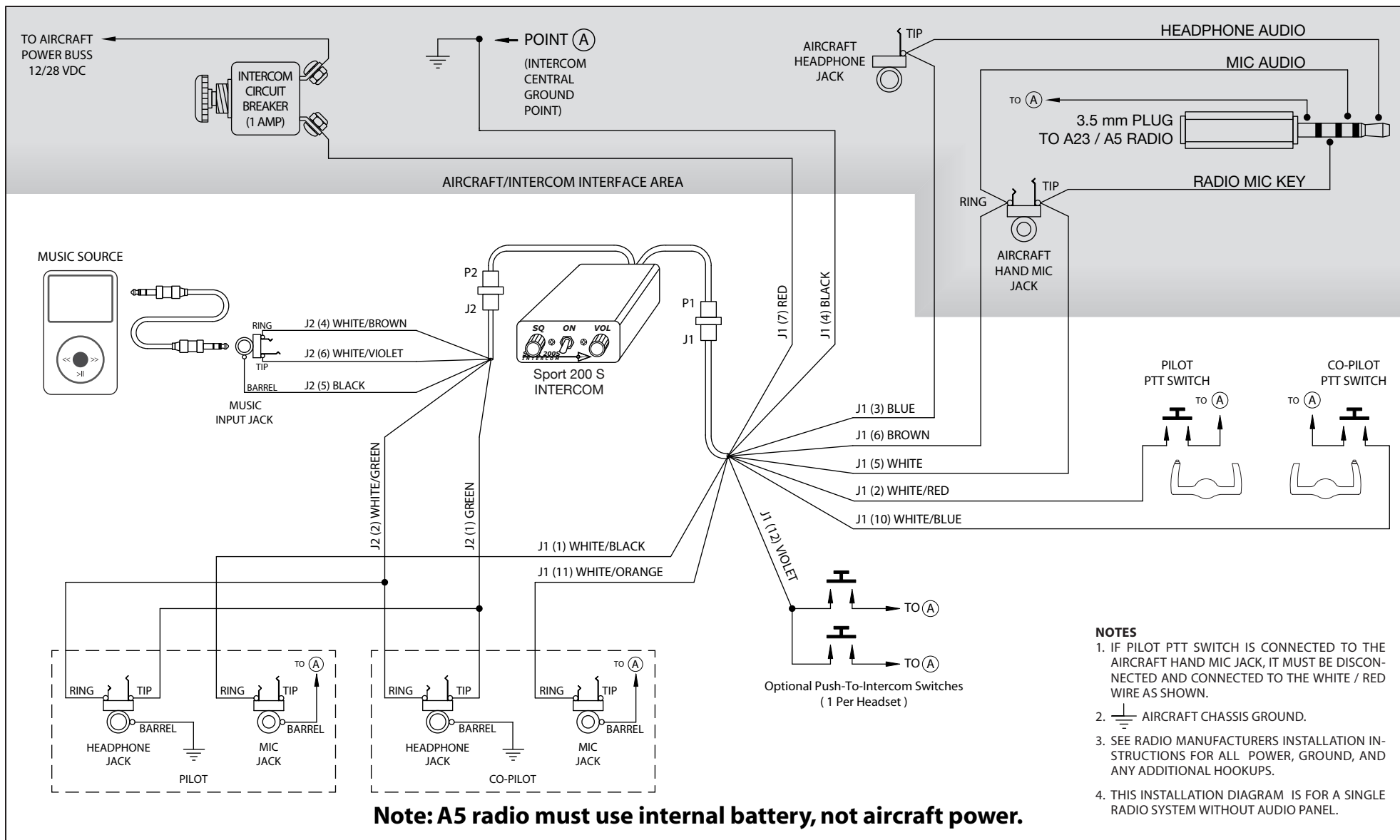
Sport 200S – ICOM A23, A5 Radio Installation Wiring Diagram
